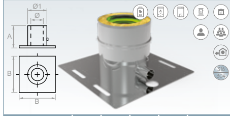
Base (Inox 316/304)
