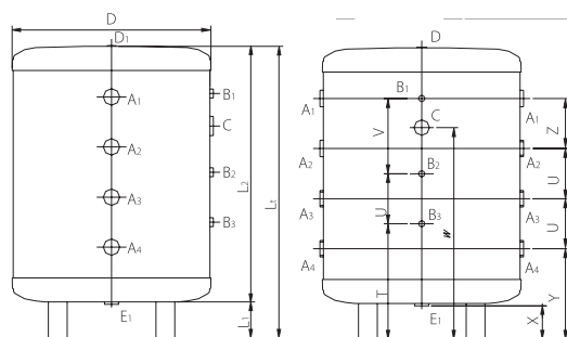
BT 100 a 250
